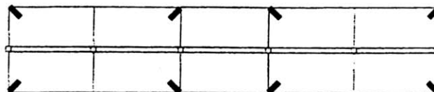
SIX UPRIGHTS...requires EIGHT ANCHORS
