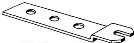
SFA-RD SEISMIC FLOOR ANCHOR regular duty...to prevent skating • Two 3/8"-16 x 3 1/2" expansion bolts per anchor
